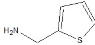
thiophene-2-methylamine
